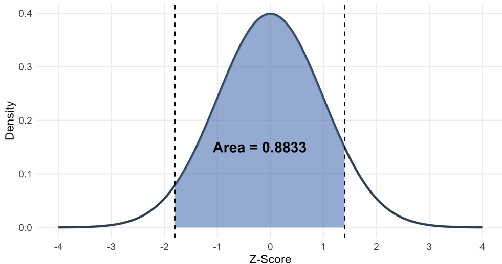
Standard Normal Curve: Area between z = -1.8 and z = 1.4
